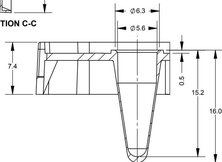
DETAIL B
