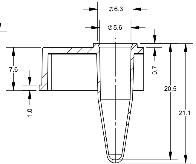
DETAIL B
