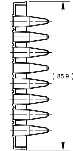
SECTION C-C
