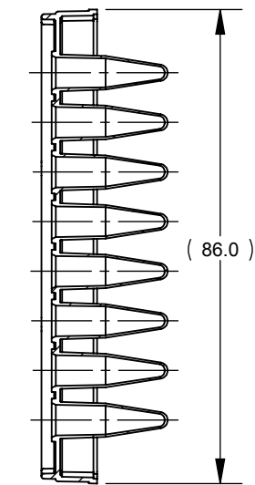
SECTION C-C
