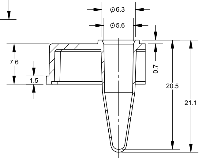
DETAIL B
